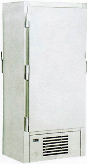
EXTERIOR VIEW - 82" HIGH MODEL Overall size: 36"Wx24"Dx82"H Power requirements: 115VAC, 60Hz, dedicated 15 amp circuit (Choose from multiple door insert options)
