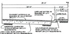
TYPICAL INTERIOR STREET 1/2 SECTION - 50' R/W NO SCALE
