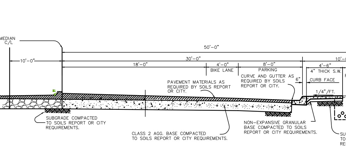
LEGAKES AVE. 1/2 SECTION - 100' R/W
