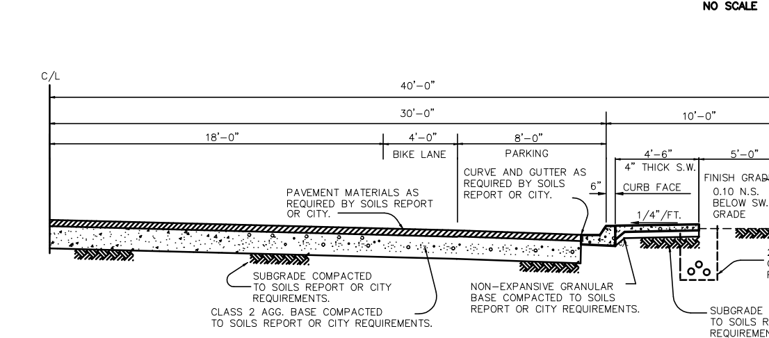
DE PAOLI STREET 1/2 SECTION - 80' R/W
