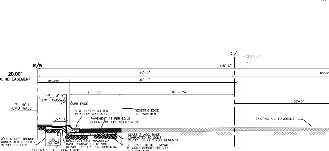
ATEN ROAD CROSS SECTION - 115' R/W
